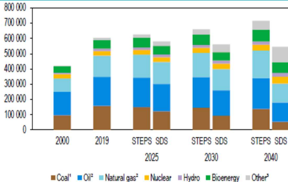
Total energy supply outlook by fuel and scenario, 2000-2040 (PJ)
